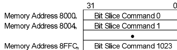
Figure B-1 Bit Slice Command Memory Addressing
