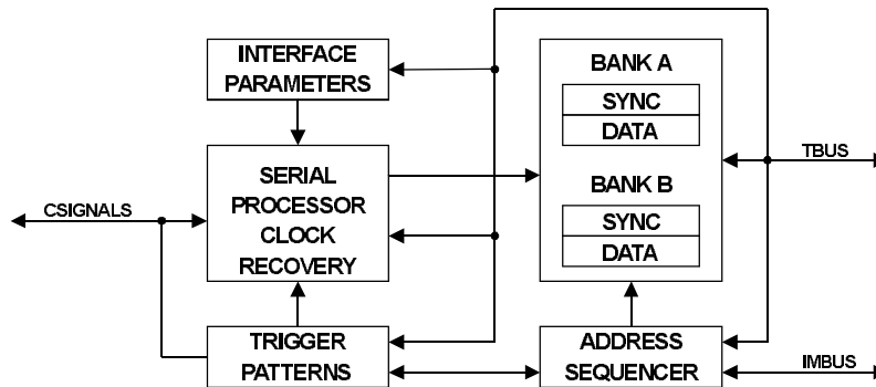
Figure 4-5 2108RX Block Diagram
