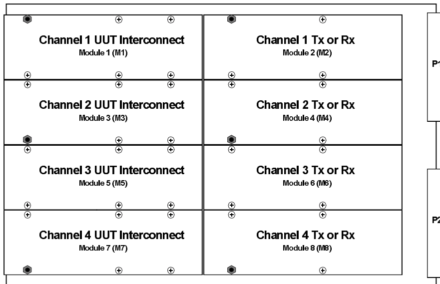
Figure 3-6 2108 Channel Module Positions
