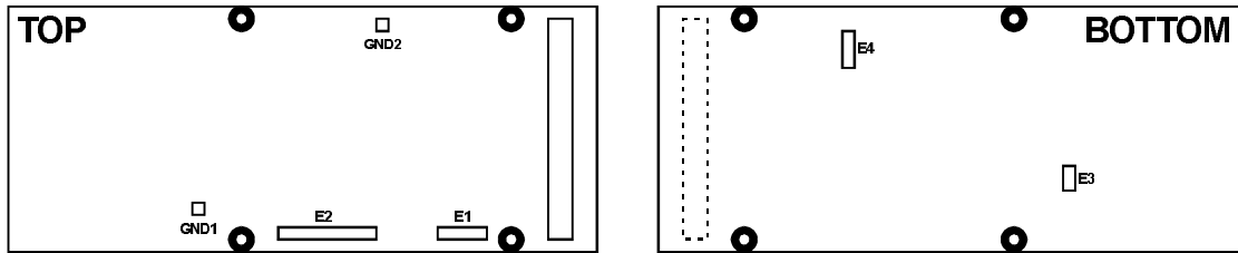
Figure 3-5 2108Tx Jumpers/Test Point Locations
