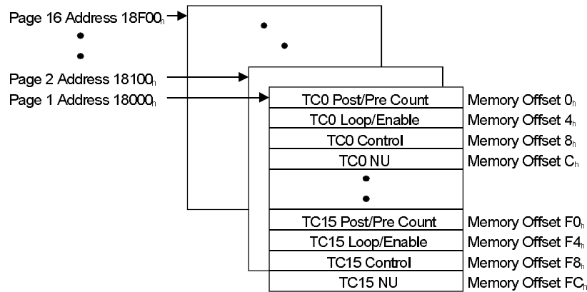
Figure B-11 Trigger Command Memory Addressing
