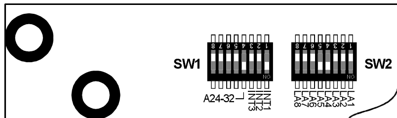
Figure 3-3 2108 Baseboard Switch Illustration
