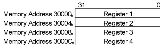
Figure B-15 Clock Generation Registers
