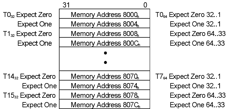
Figure B-10 Bit Slice Memory Addressing
