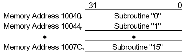
Figure B-2 Subroutine Memory Addressing
