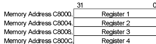
Figure B-7 Clock Generation Registers
