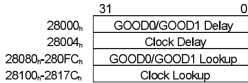
Figure B-14 ReceiverDelay Control Memory
